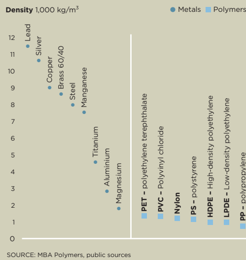
FIGURE 19 Metals can easily be distinguished by density and other physical properties, while polymers cannot
