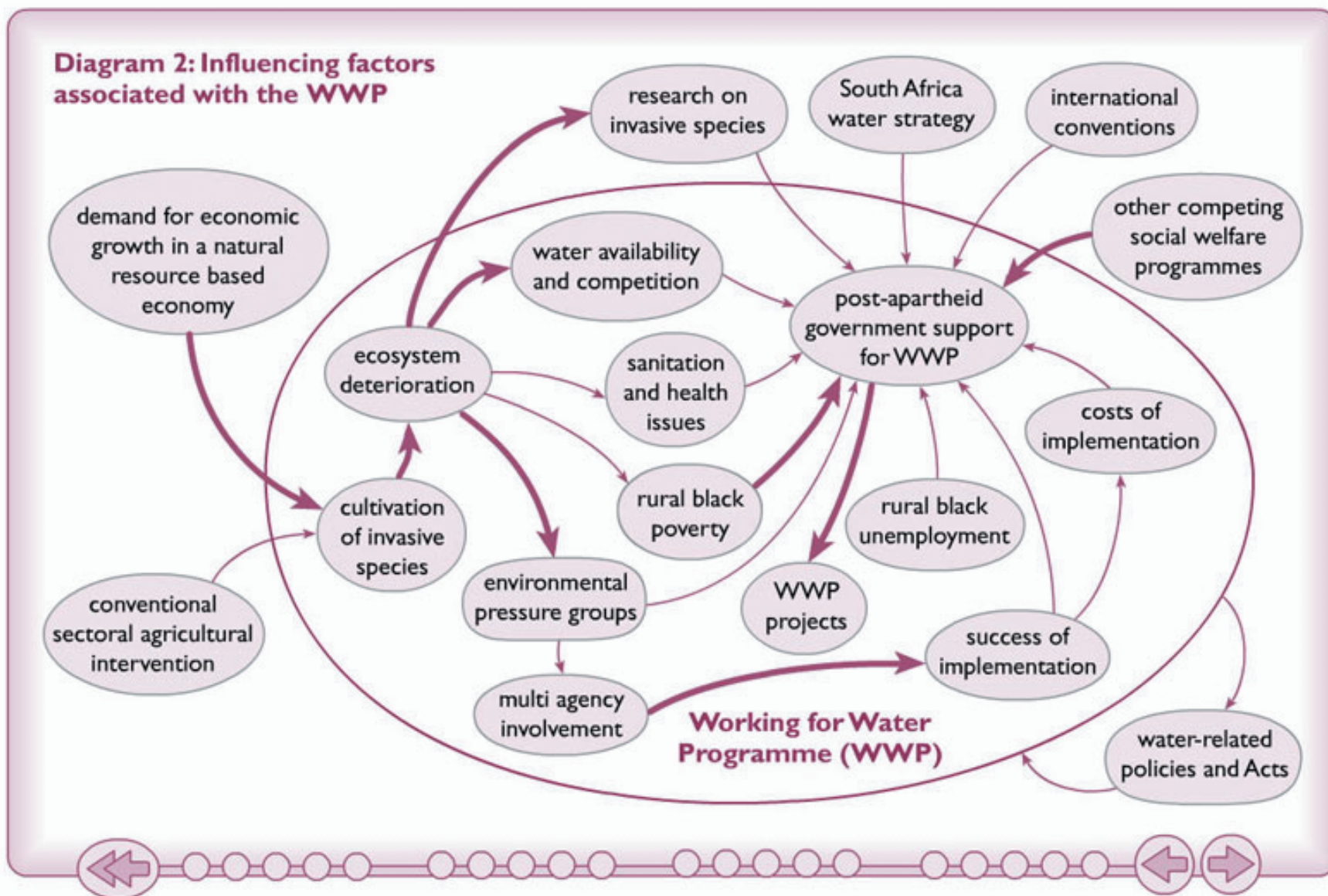
Influence diagram 2
