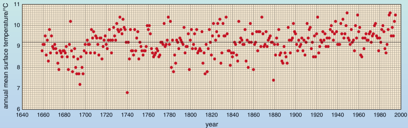
Figure 2.10 The central England temperature record from 1659 to 1995. Each year is represented by a single dot giving the annual mean surface temperature for that year. The 1659–1995 mean temperature of 9.2 °C is indicated by the horizontal line.
