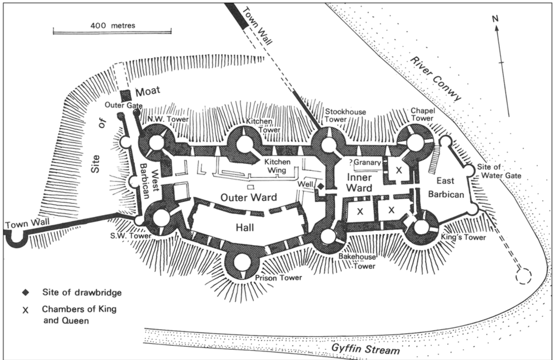
Plan of Conwy Castle
